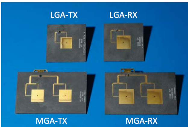
X-band Patch Antennas
