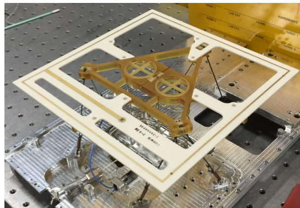
UHF Loop Antenna
